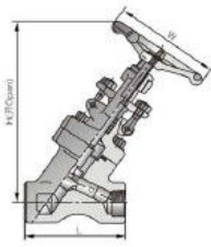
螺栓连接阀盖, 缩径和全径, 明杆支架 (OS&Y) Bolted bonnet, full port reducing port outside screw and yoke(OS & Y) 末端连接为螺纹或承插焊对接, 设计按BS5352 Threaded, butt-welded or socket welded ends; design to BS5352
